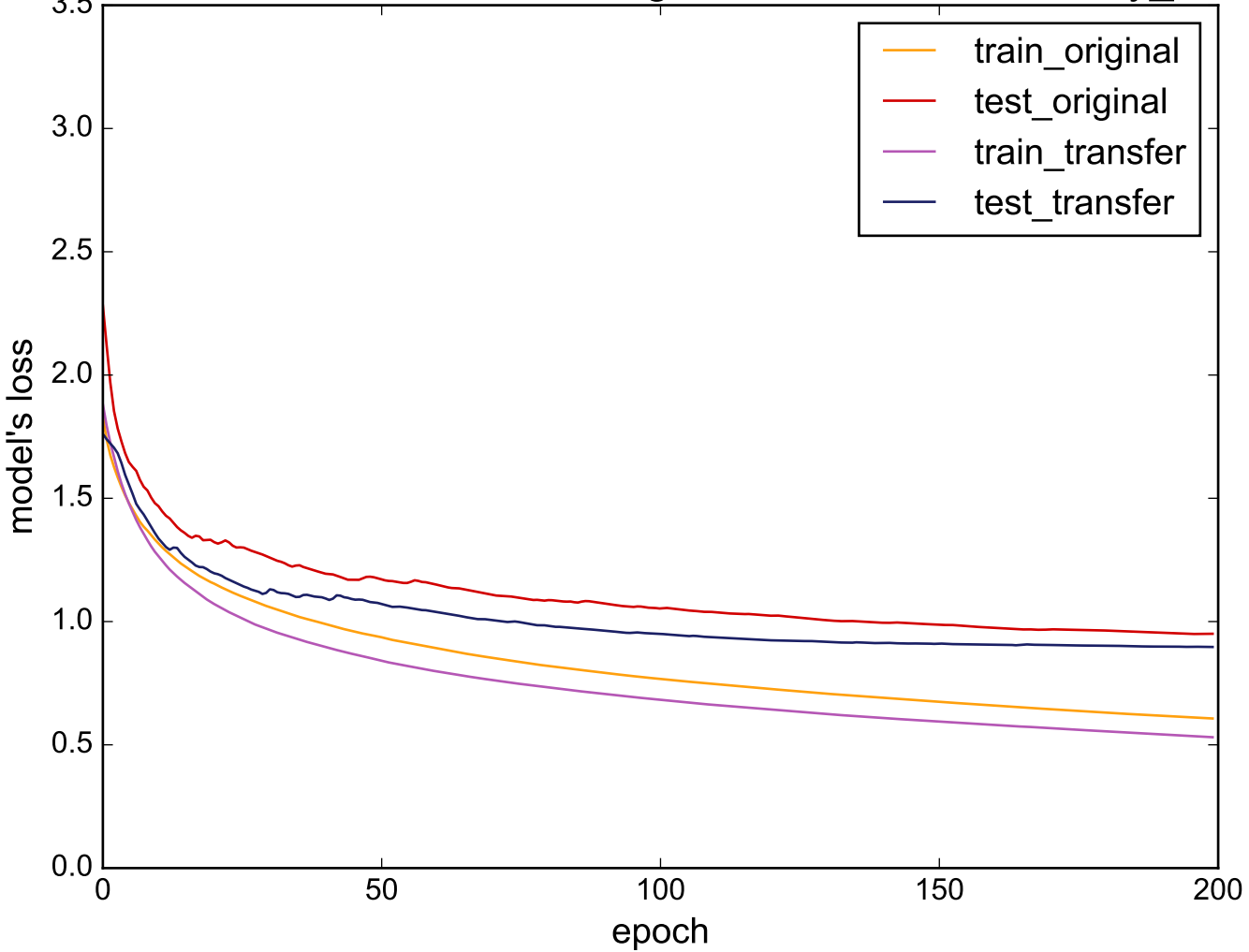
Source: HandOutlines - Target: uWaveGestureLibrary_X
