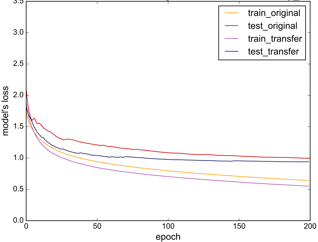
Source: HandOutlines - Target: uWaveGestureLibrary_Z
