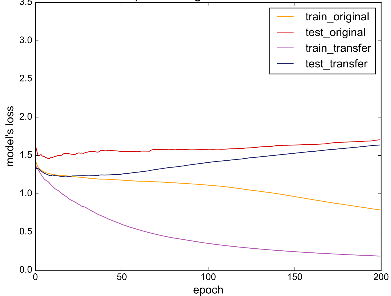
Source: Haptics - Target: DiatomSizeReduction
