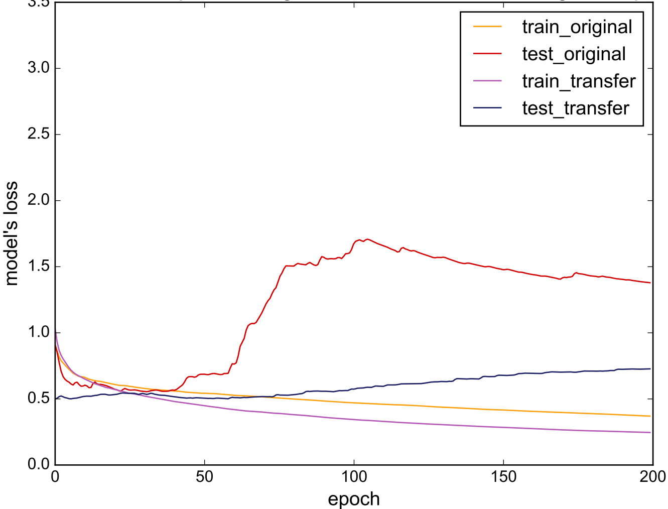
Source: Haptics - Target: DistalPhalanxOutlineAgeGroup
