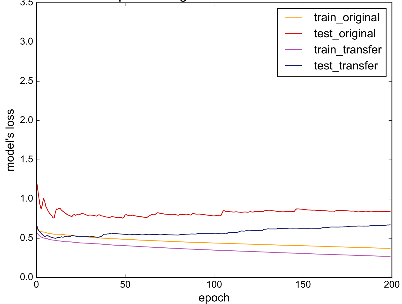
Source: Haptics - Target: DistalPhalanxOutlineCorrect
