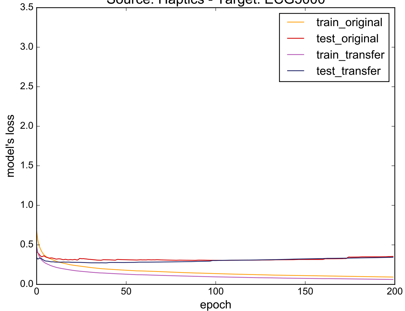
Source: Haptics - Target: ECG5000
