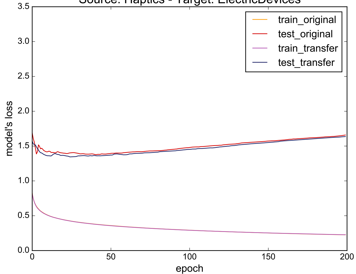
Source: Haptics - Target: ElectricDevices
