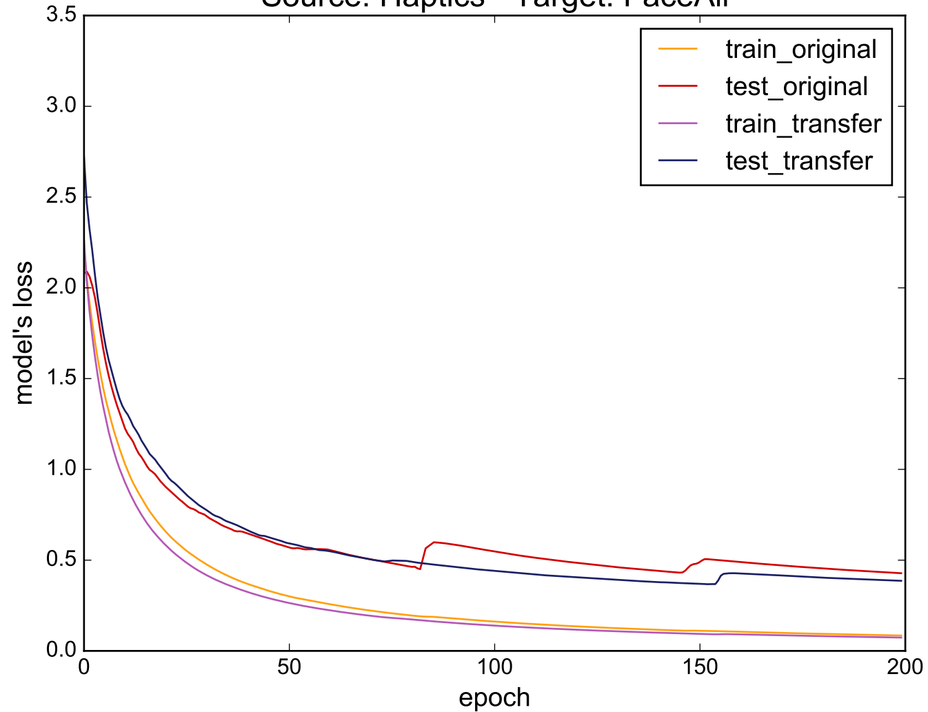
Source: Haptics - Target: FaceAll
