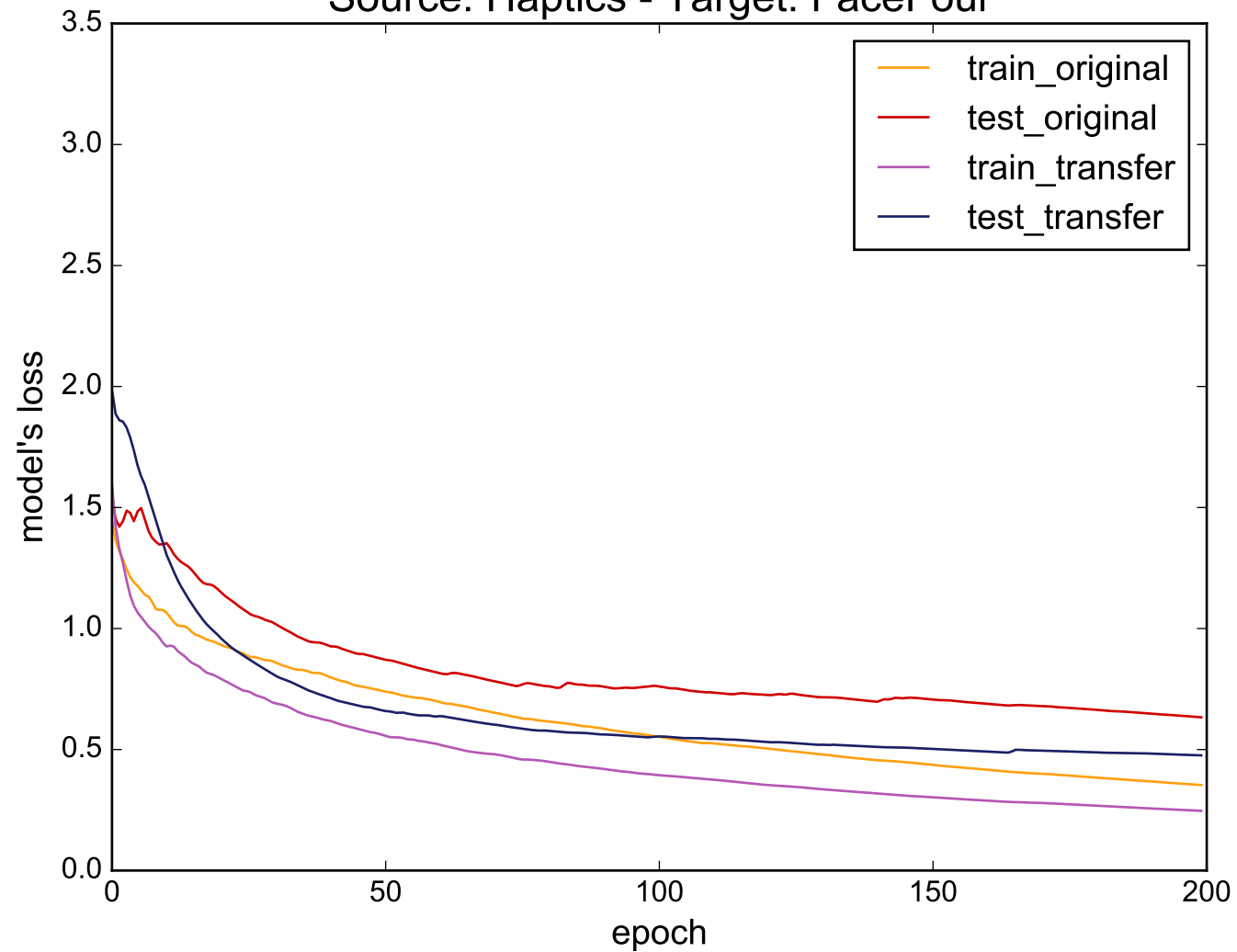
Source: Haptics - Target: FaceFour
