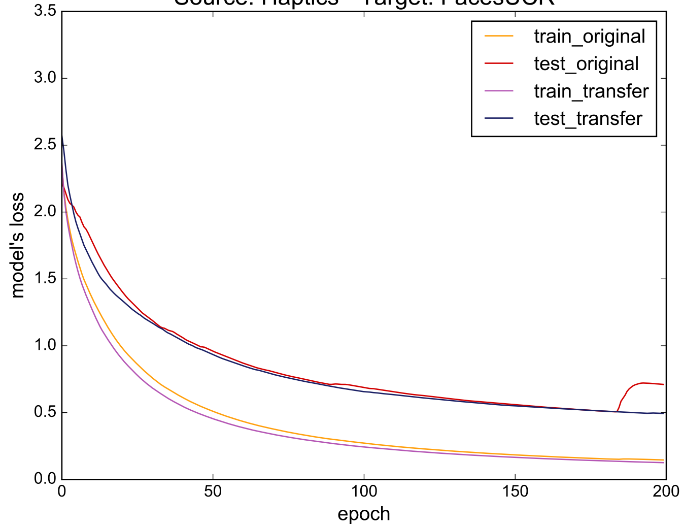
Source: Haptics - Target: FacesUCR
