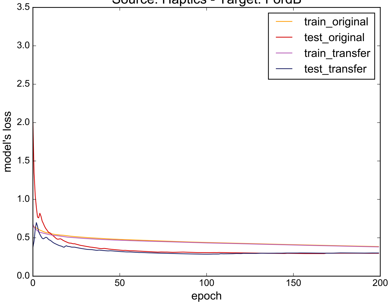
Source: Haptics - Target: FordB
