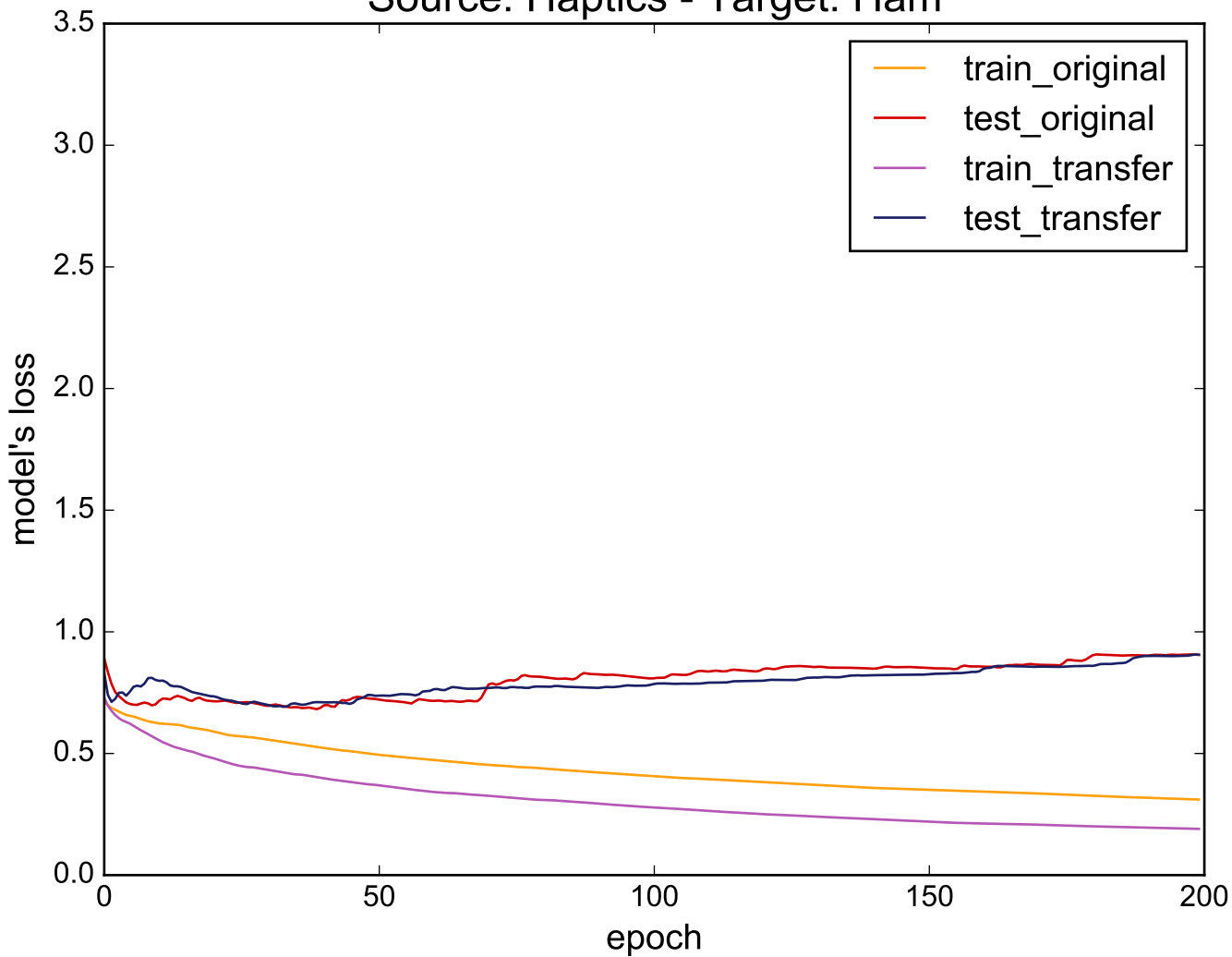
Source: Haptics - Target: Ham
