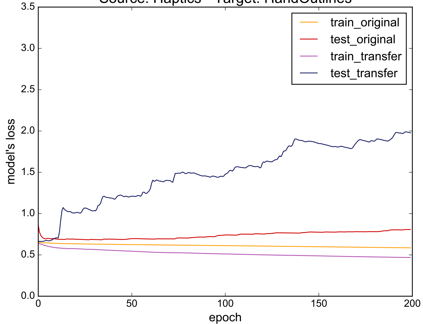
Source: Haptics - Target: HandOutlines
