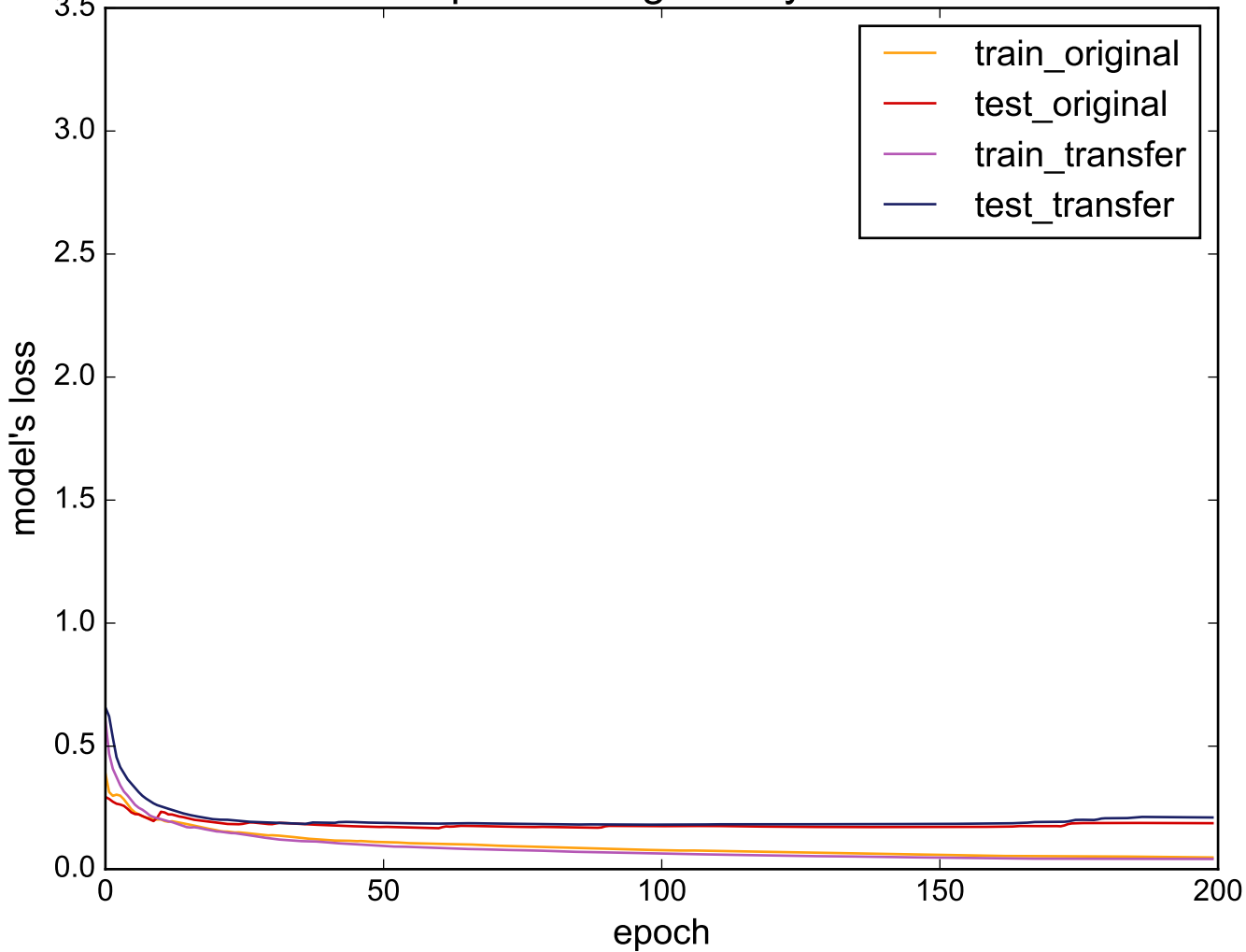
Source: Haptics - Target: ItalyPowerDemand
