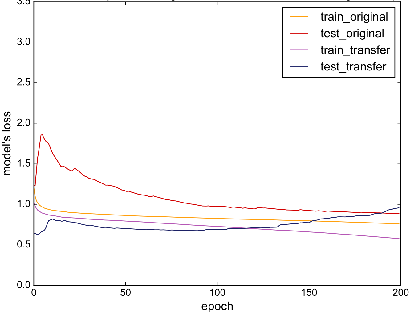
Source: Haptics - Target: MiddlePhalanxOutlineAgeGroup
