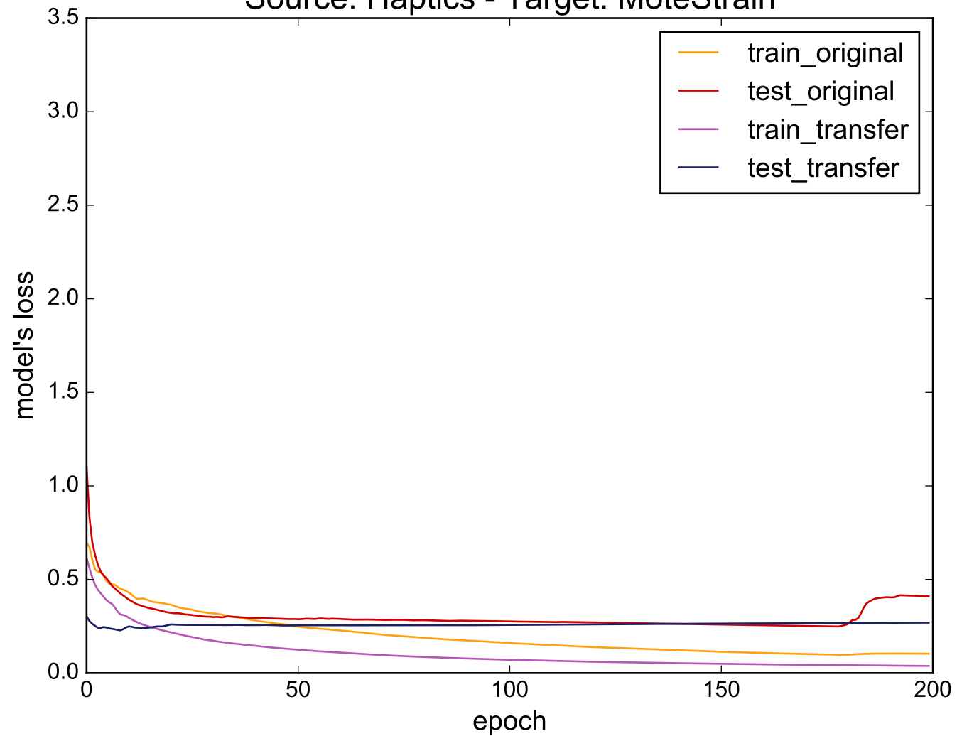
Source: Haptics - Target: MoteStrain
