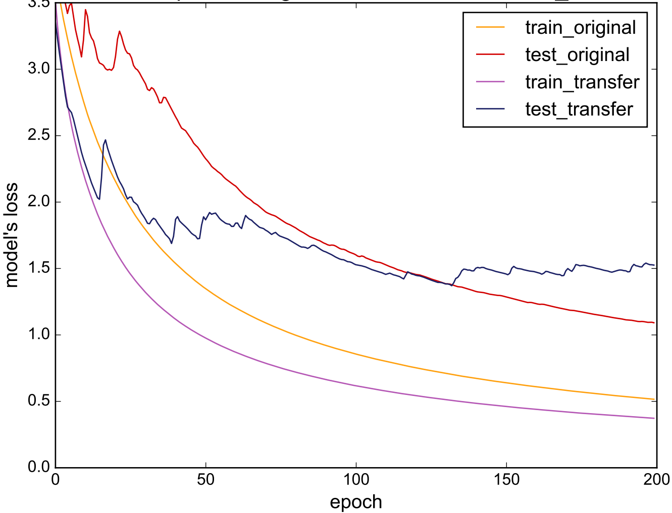
Source: Haptics - Target: NonInvasiveFetalECG_Thorax1
