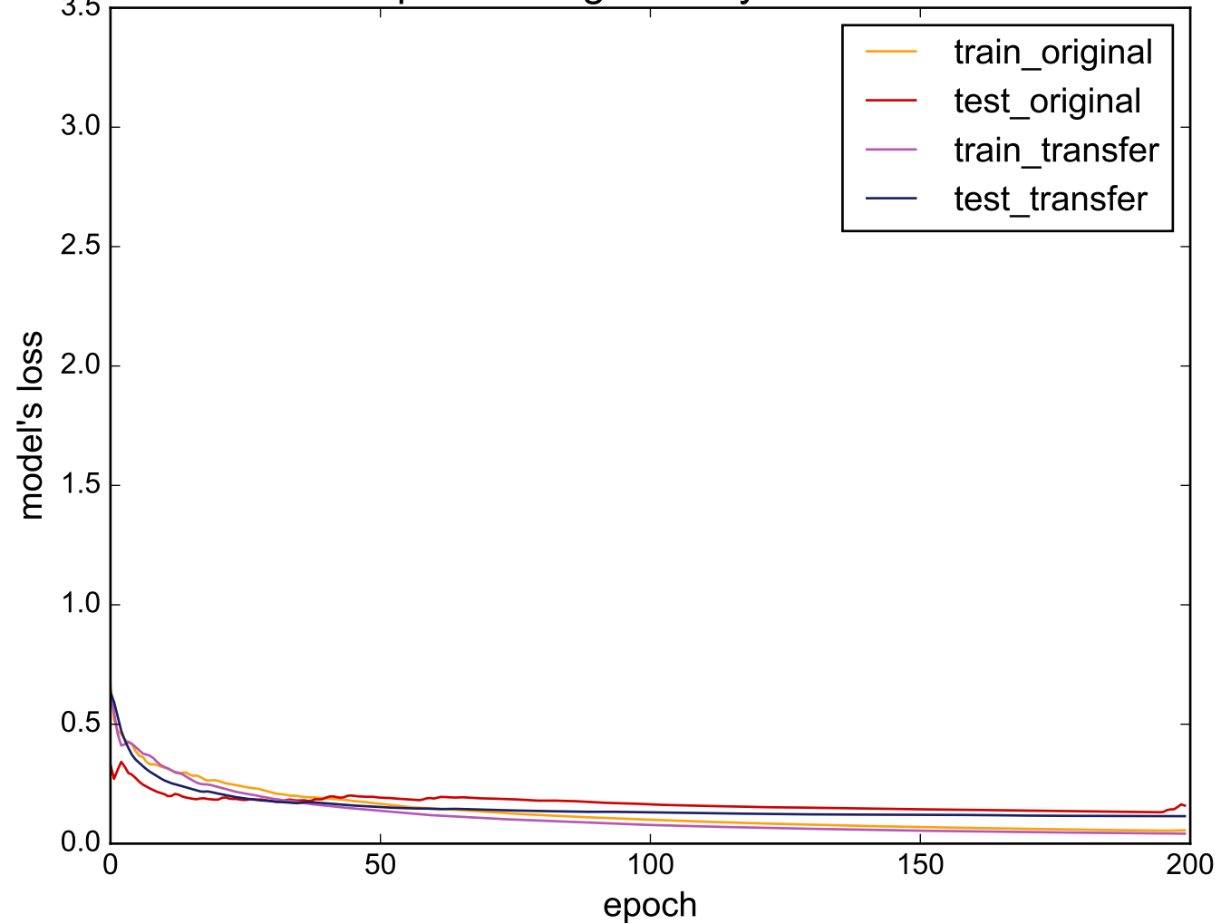
Source: Haptics - Target: SonyAIBORobotSurface
