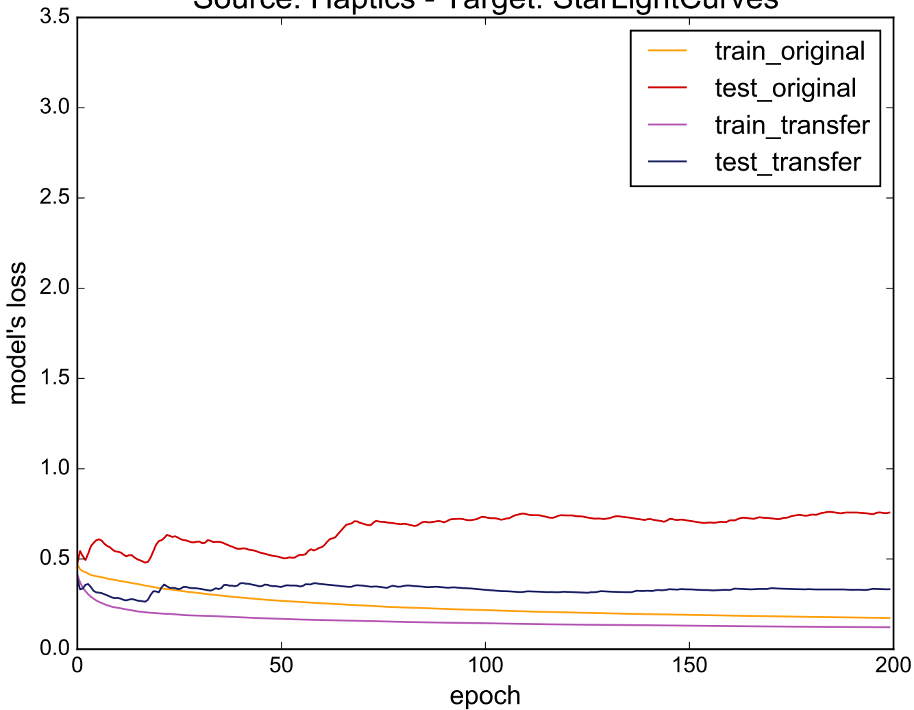
Source: Haptics - Target: StarLightCurves
