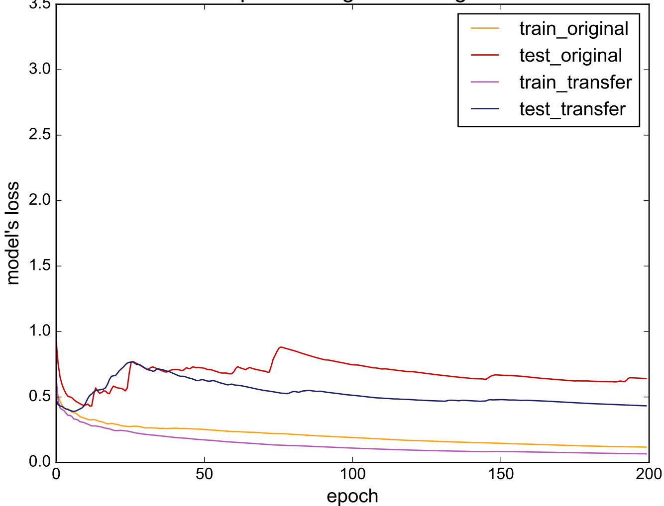
Source: Haptics - Target: ToeSegmentation2
