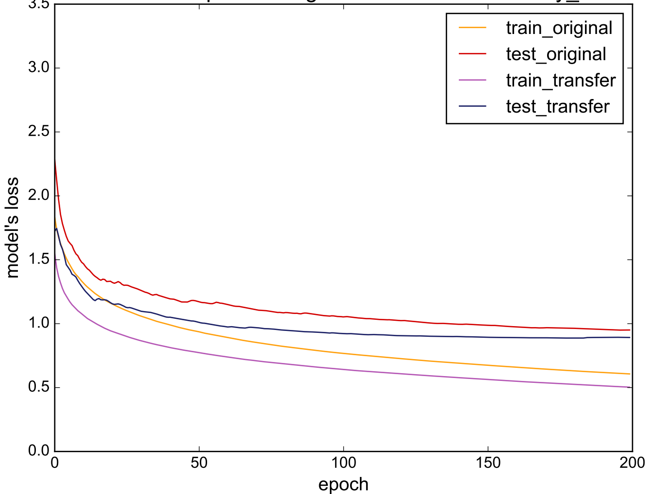
Source: Haptics - Target: uWaveGestureLibrary_X
