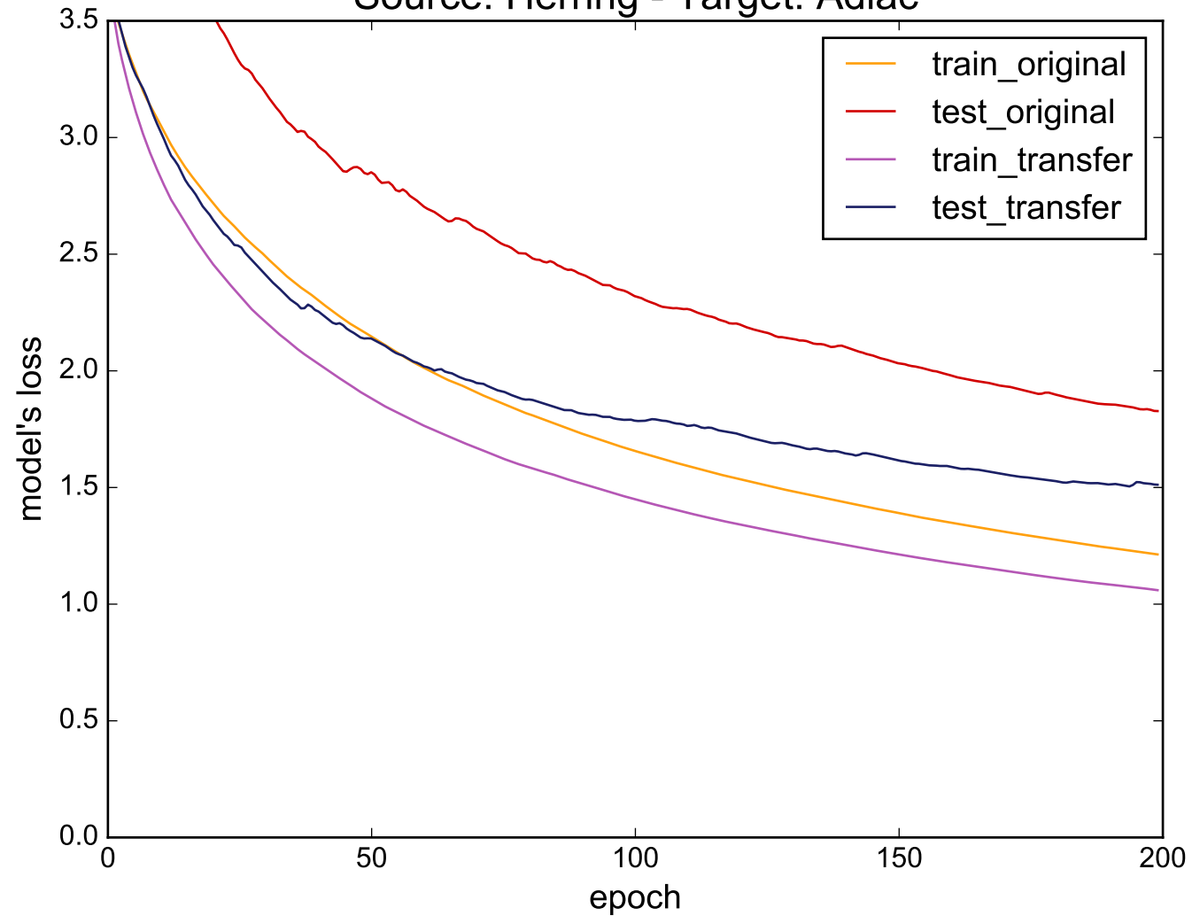
Source: Herring - Target: Adiac
