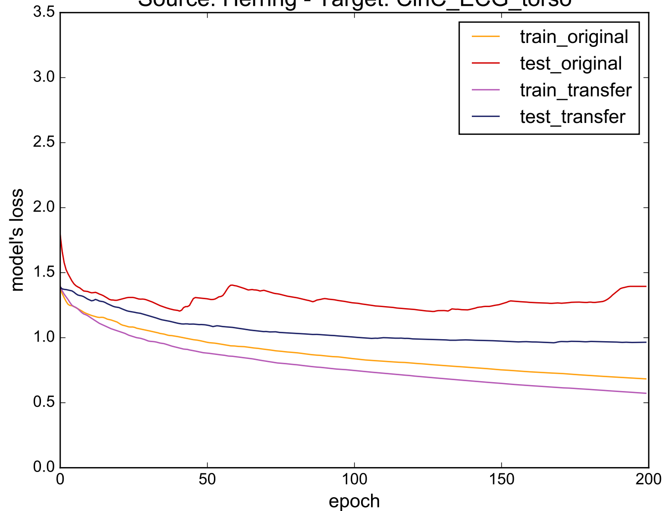
Source: Herring - Target: CinC_ECG_torso
