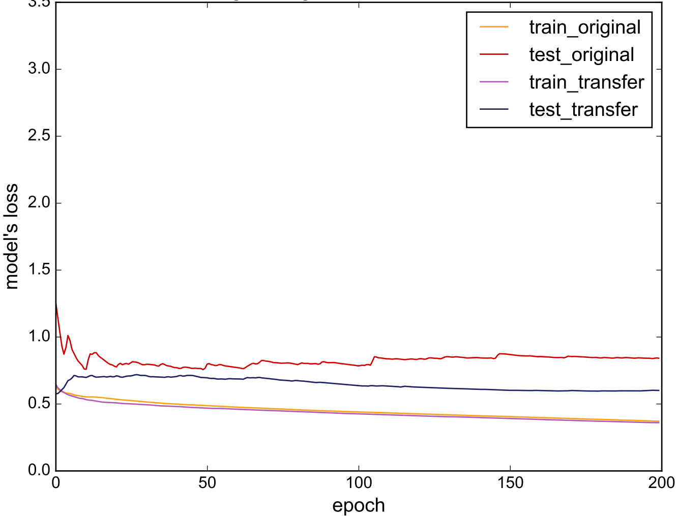
Source: Herring - Target: DistalPhalanxOutlineCorrect
