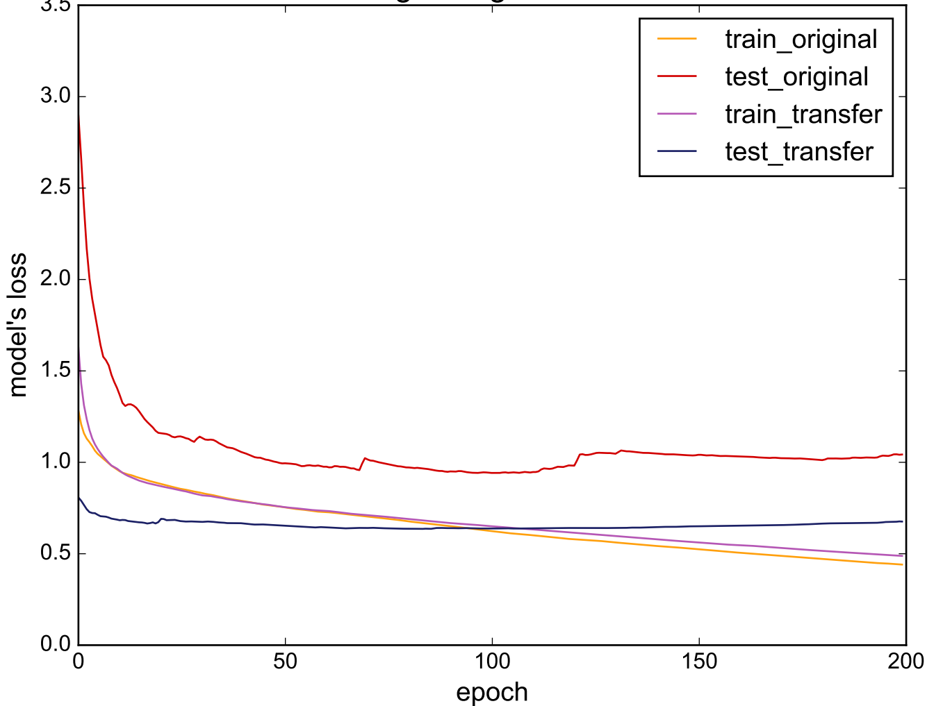
Source: Herring - Target: DistalPhalanxTW
