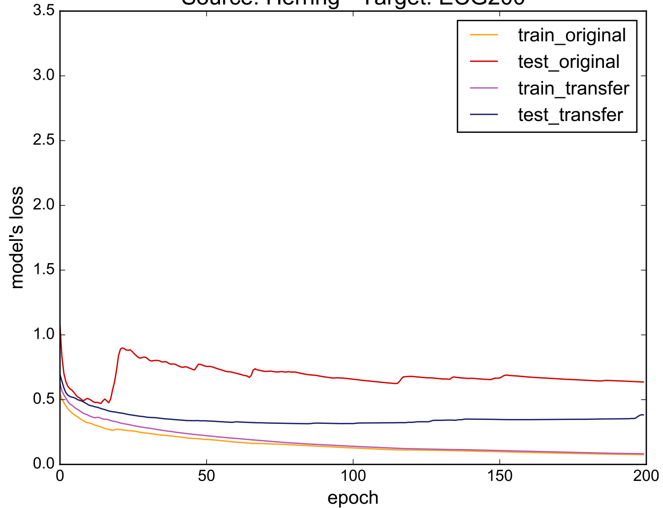
Source: Herring - Target: ECG200
