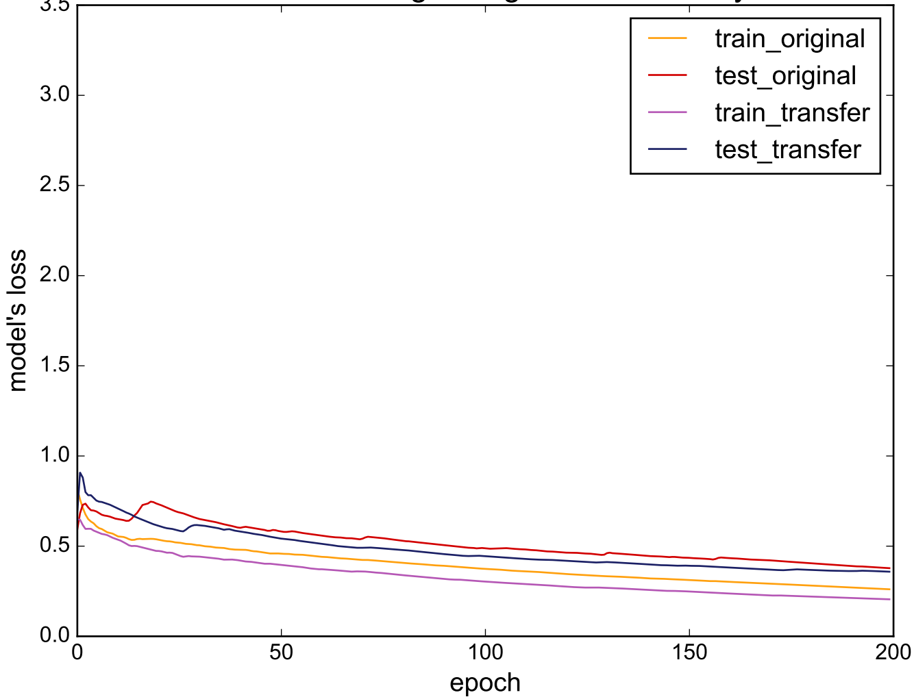
Source: Herring - Target: ECGFiveDays
