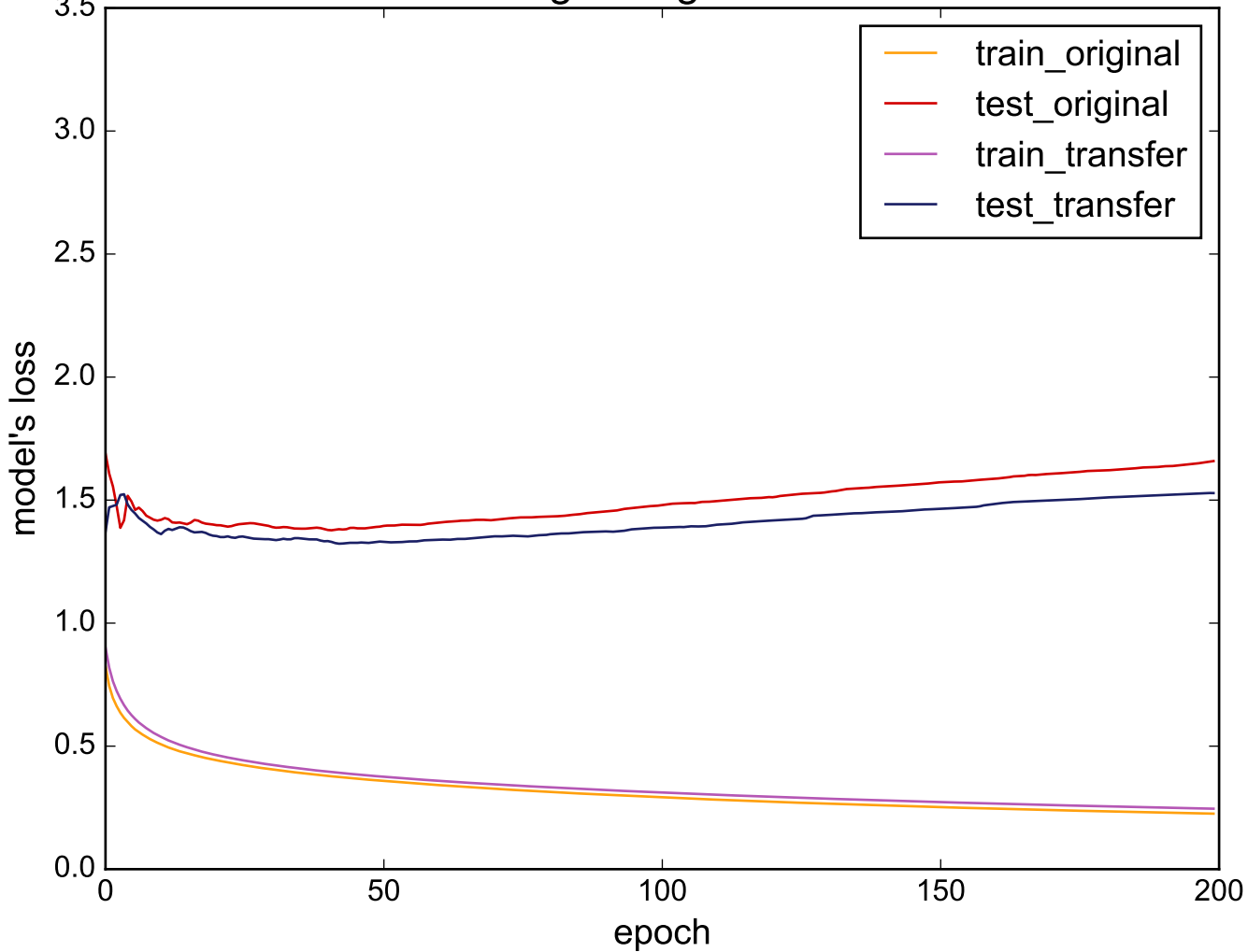
Source: Herring - Target: ElectricDevices
