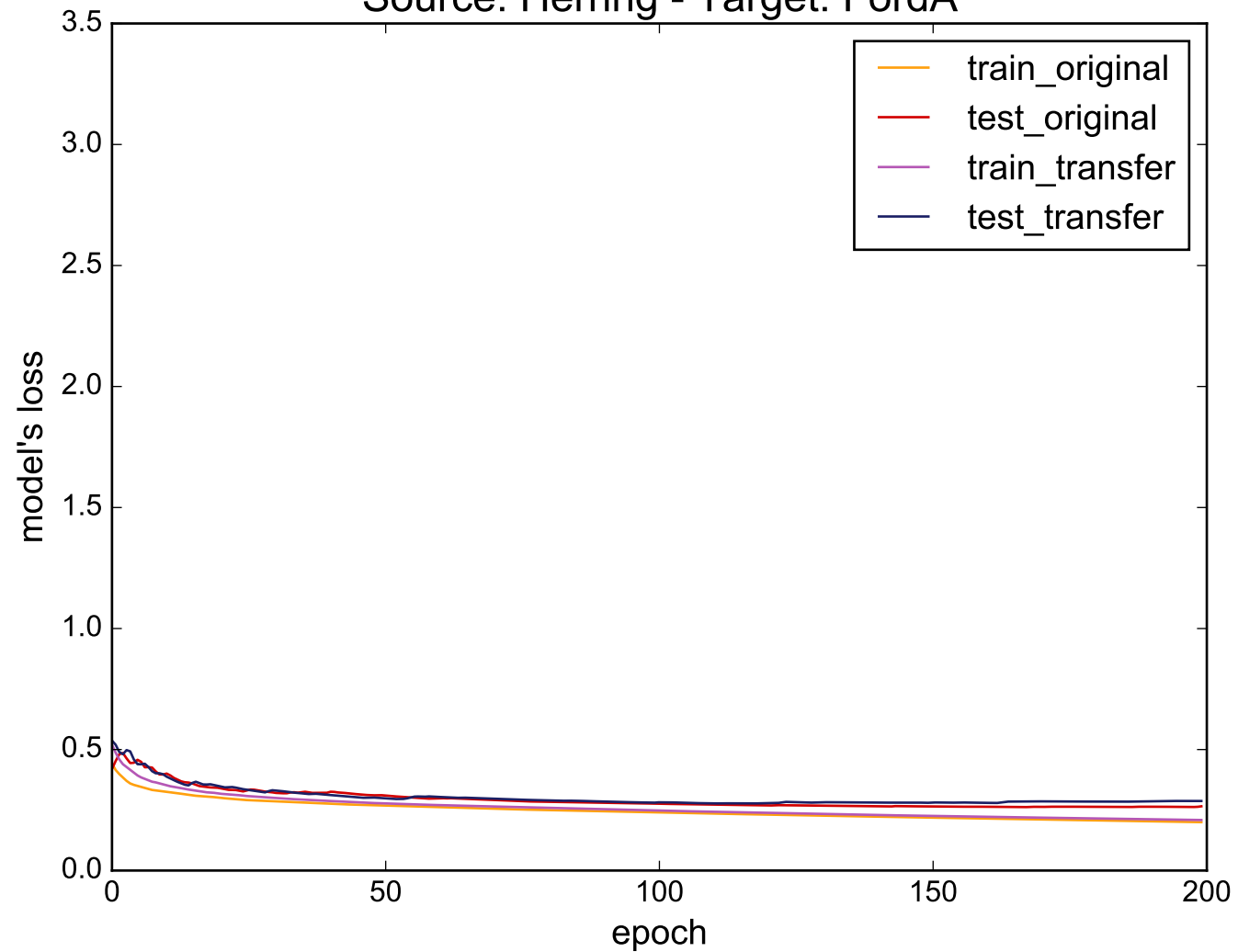
Source: Herring - Target: FordA
