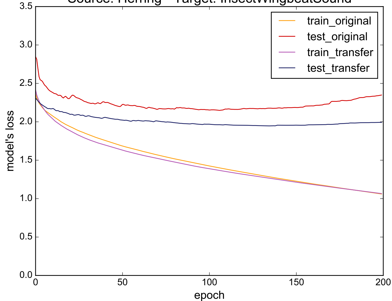
Source: Herring - Target: InsectWingbeatSound
