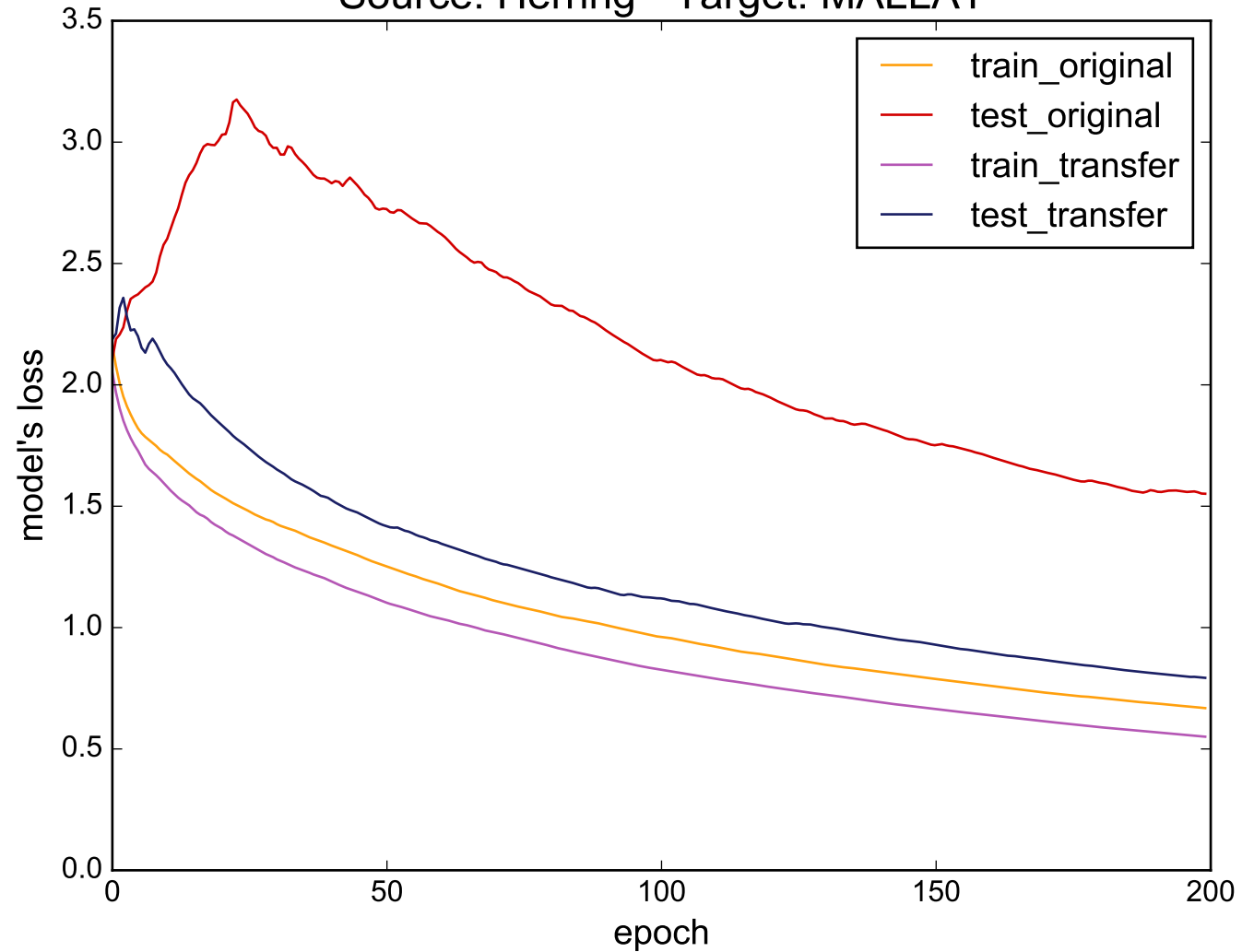
Source: Herring - Target: MALLAT
