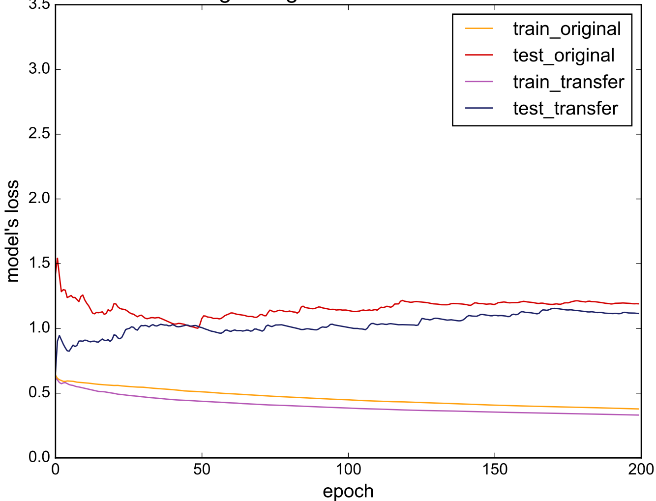
Source: Herring - Target: MiddlePhalanxOutlineCorrect
