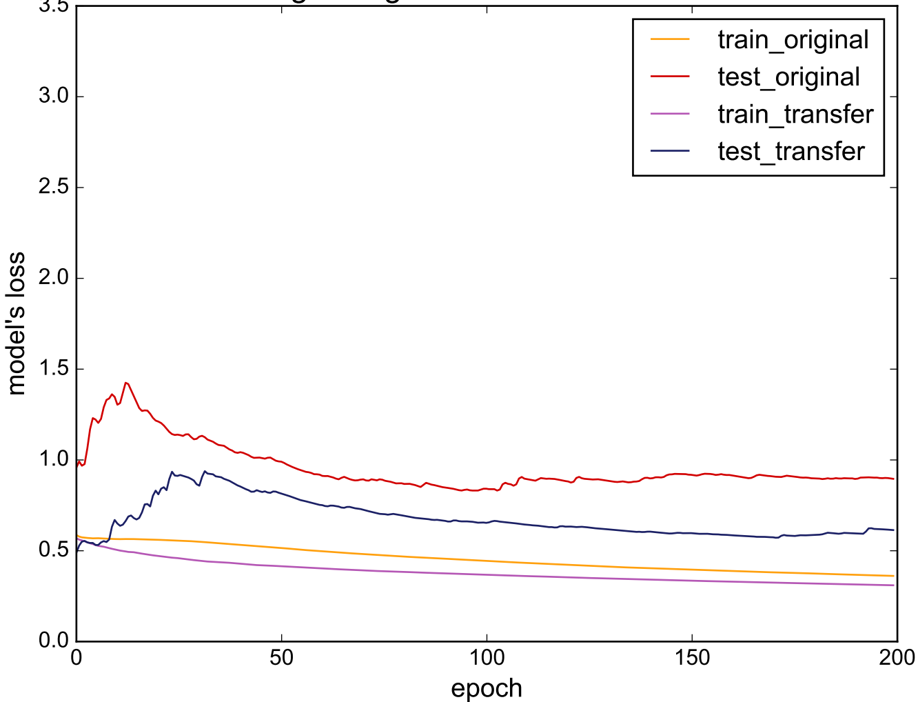
Source: Herring - Target: ProximalPhalanxOutlineCorrect
