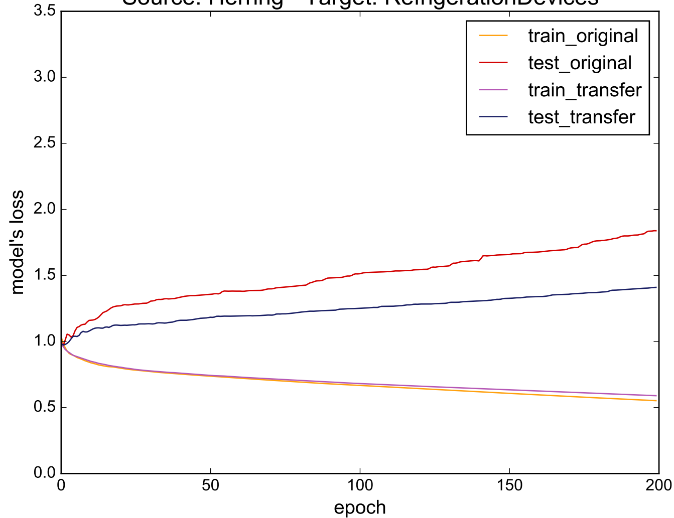
Source: Herring - Target: RefrigerationDevices
