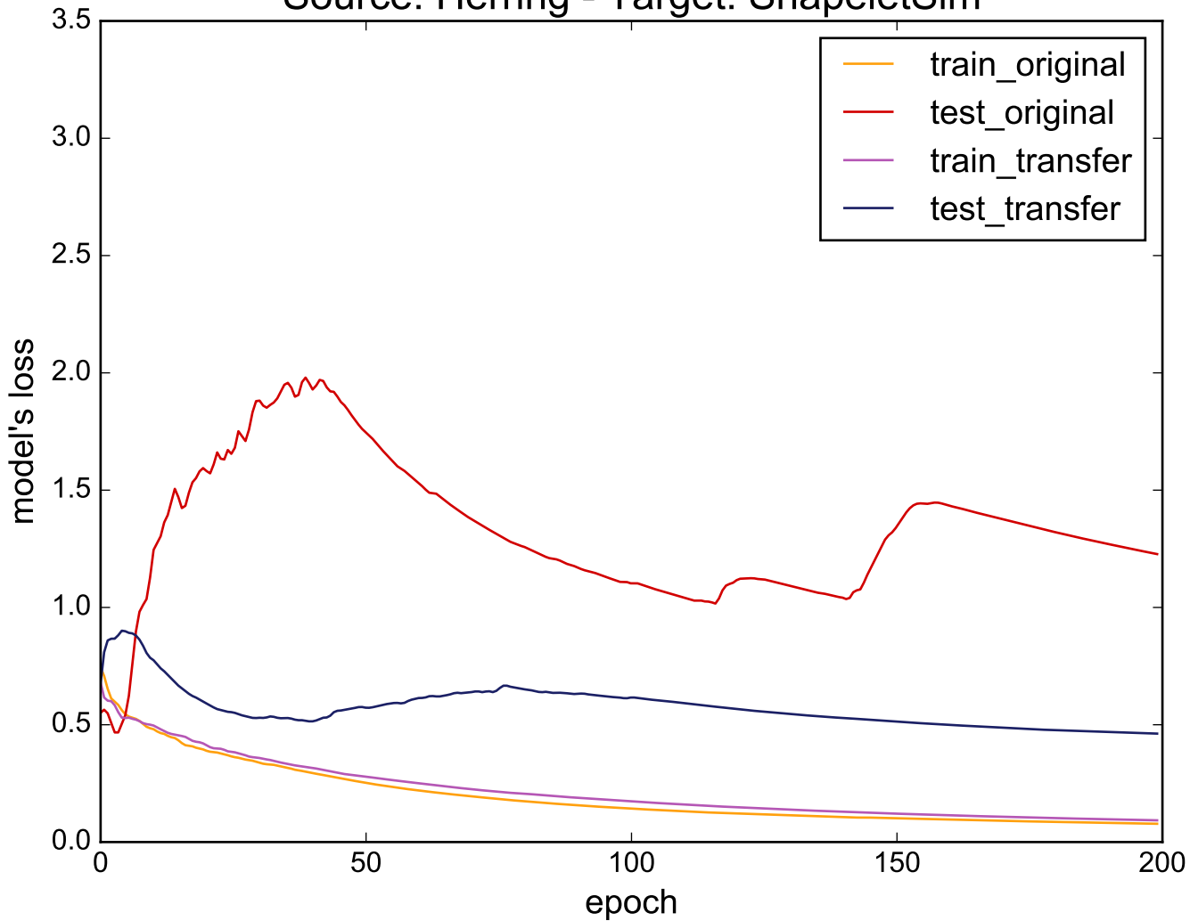
Source: Herring - Target: ShapeletSim
