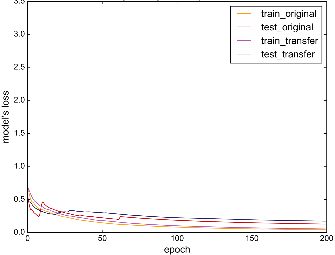
Source: Herring - Target: SonyAIBORobotSurfaceII
