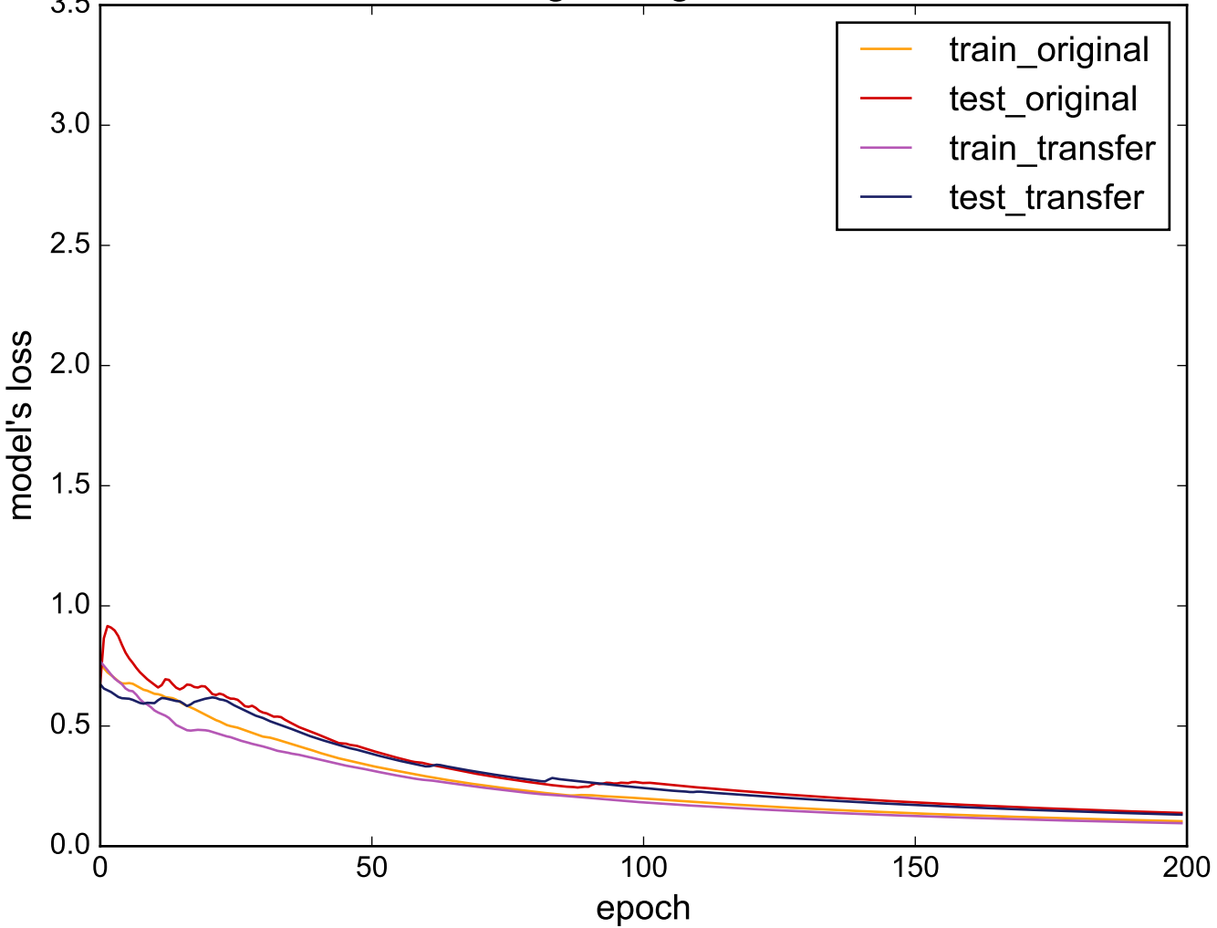
Source: Herring - Target: TwoLeadECG
