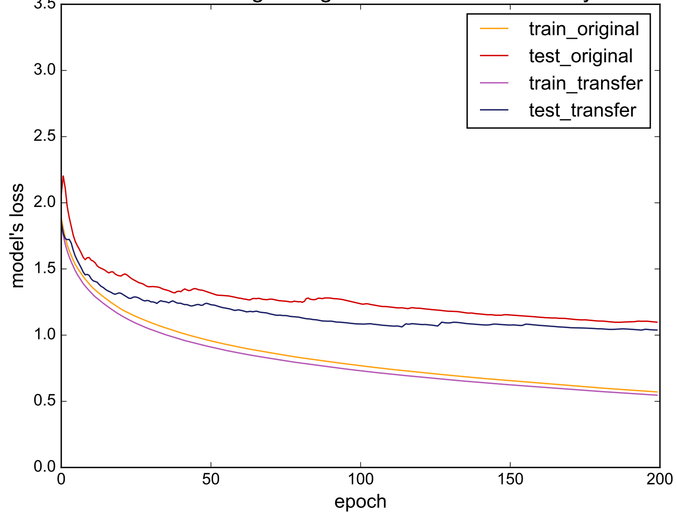
Source: Herring - Target: UWaveGestureLibraryAll
