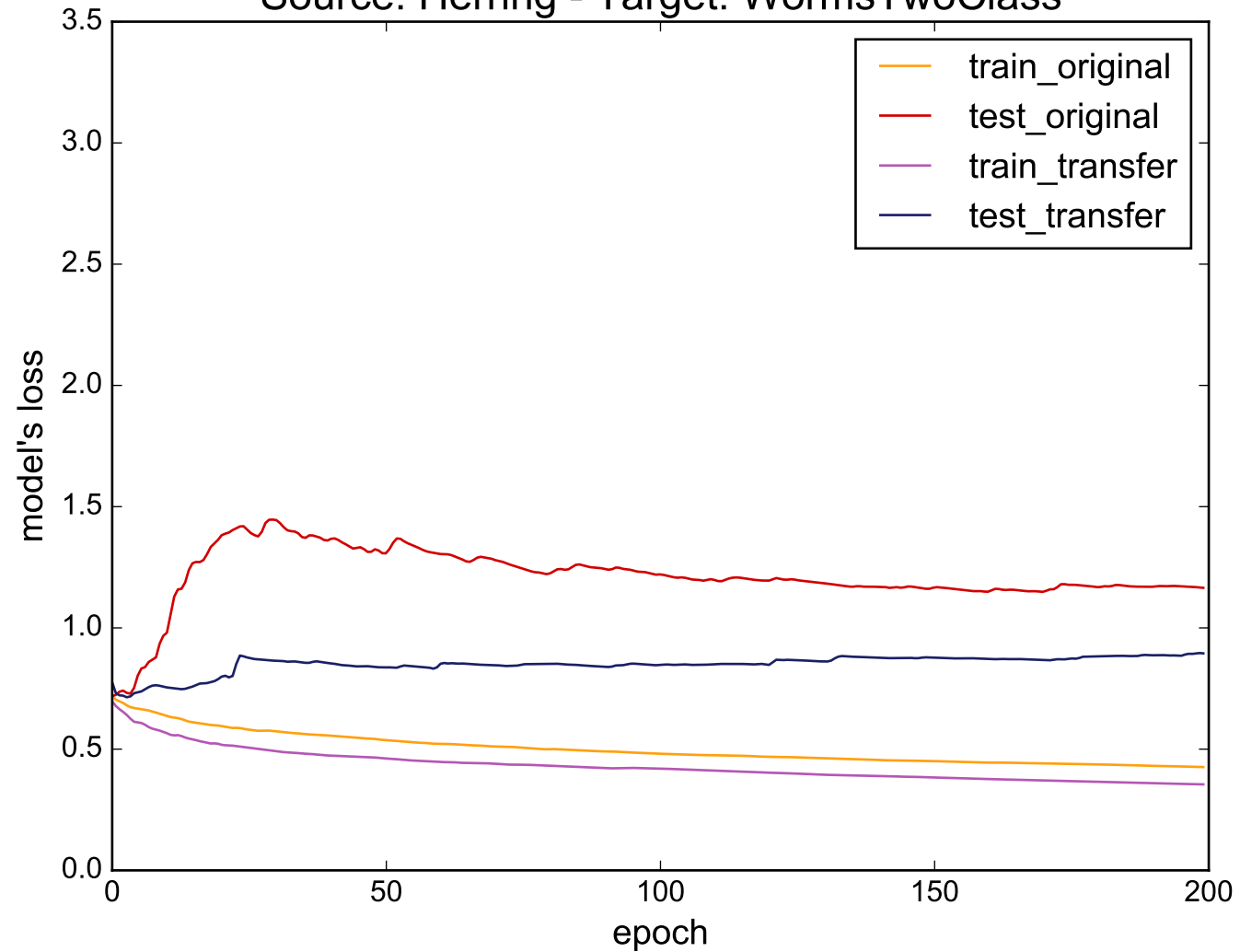
Source: Herring - Target: WormsTwoClass
