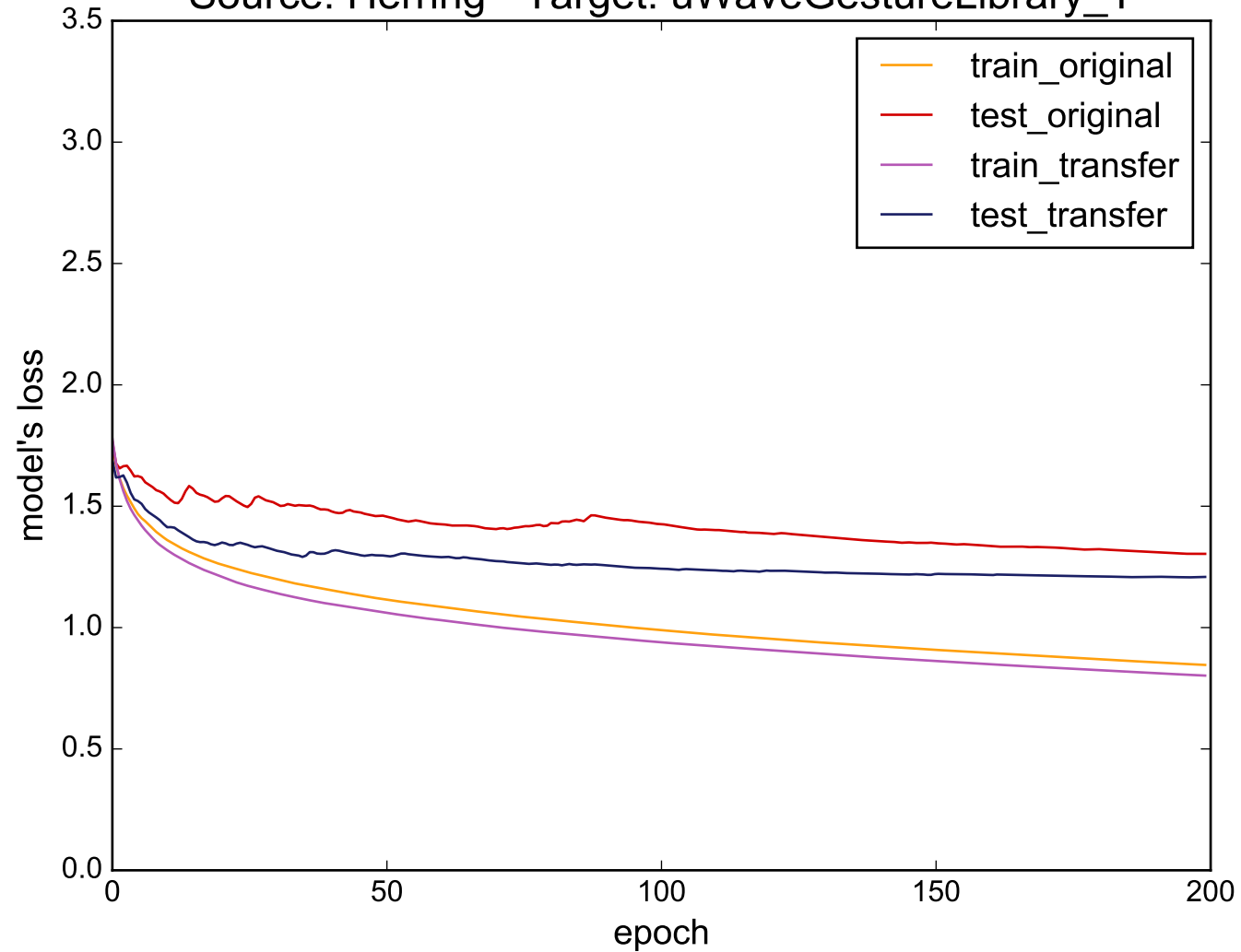
Source: Herring - Target: uWaveGestureLibrary_Y
