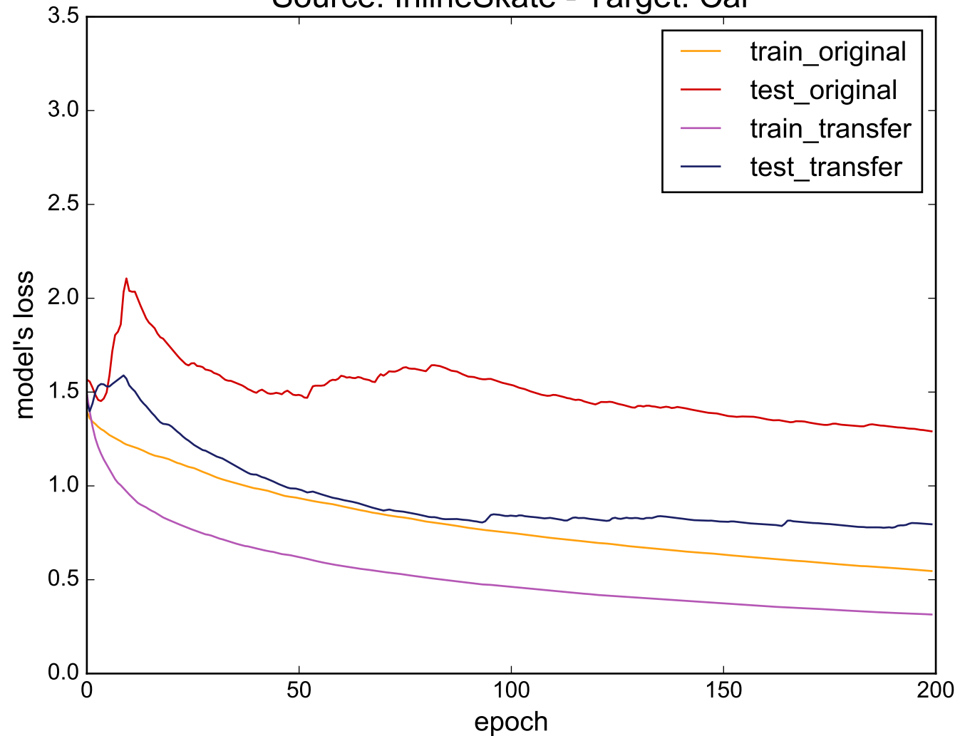
Source: InlineSkate - Target: Car
