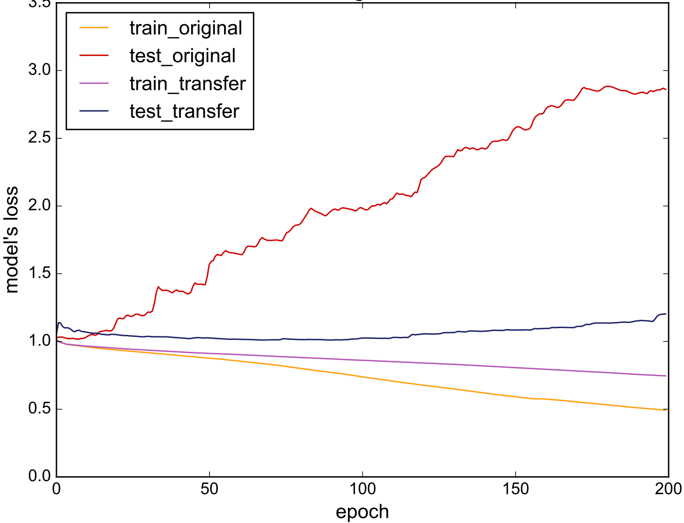
Source: InlineSkate - Target: ChlorineConcentration
