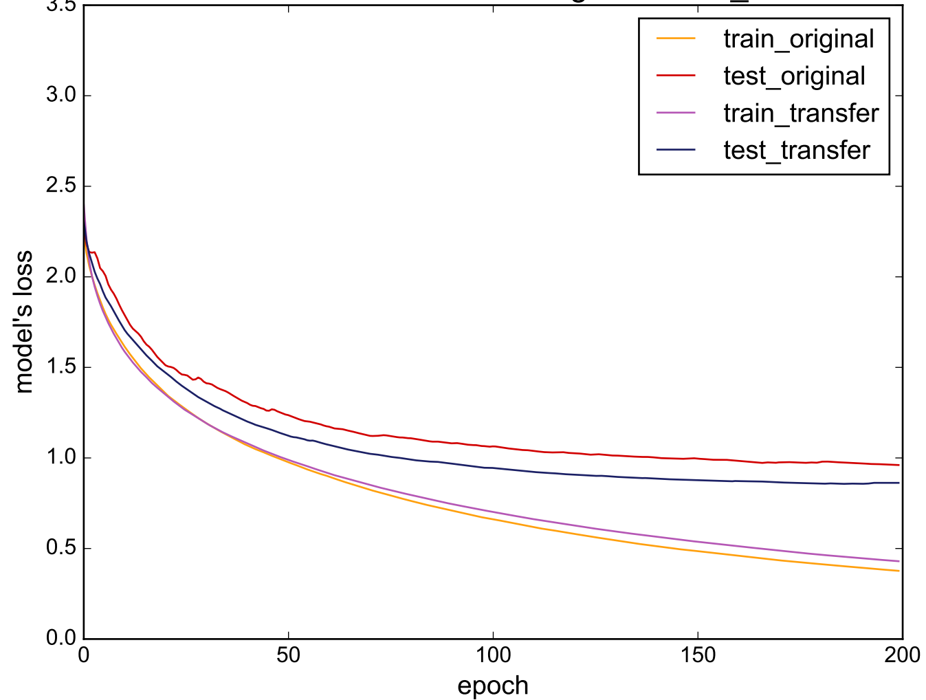
Source: InlineSkate - Target: Cricket_Z
