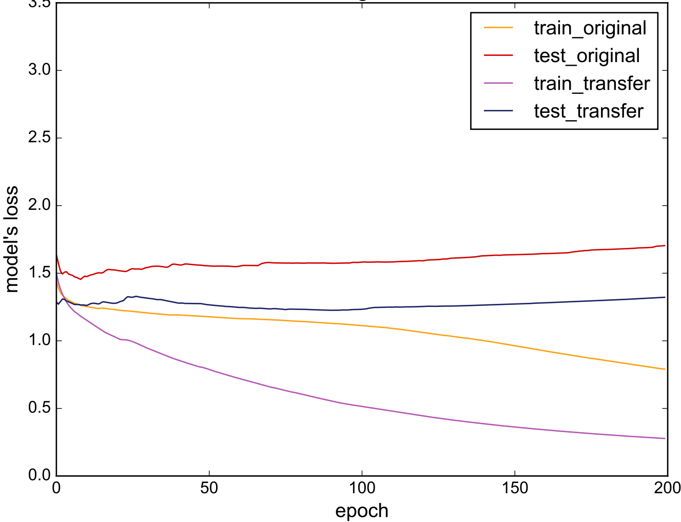
Source: InlineSkate - Target: DiatomSizeReduction
