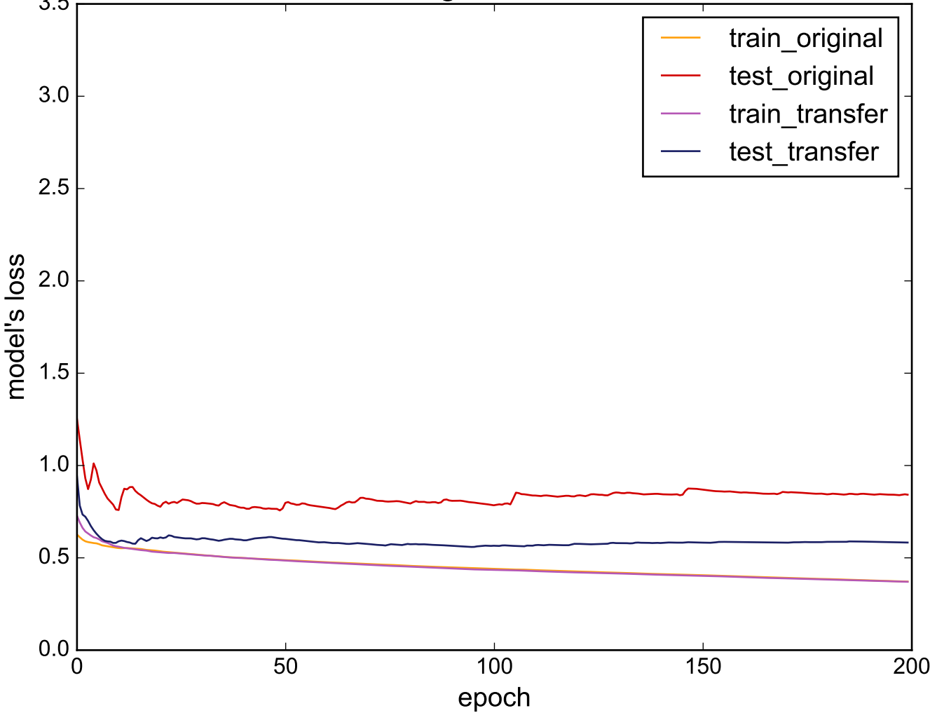
Source: InlineSkate - Target: DistalPhalanxOutlineCorrect
