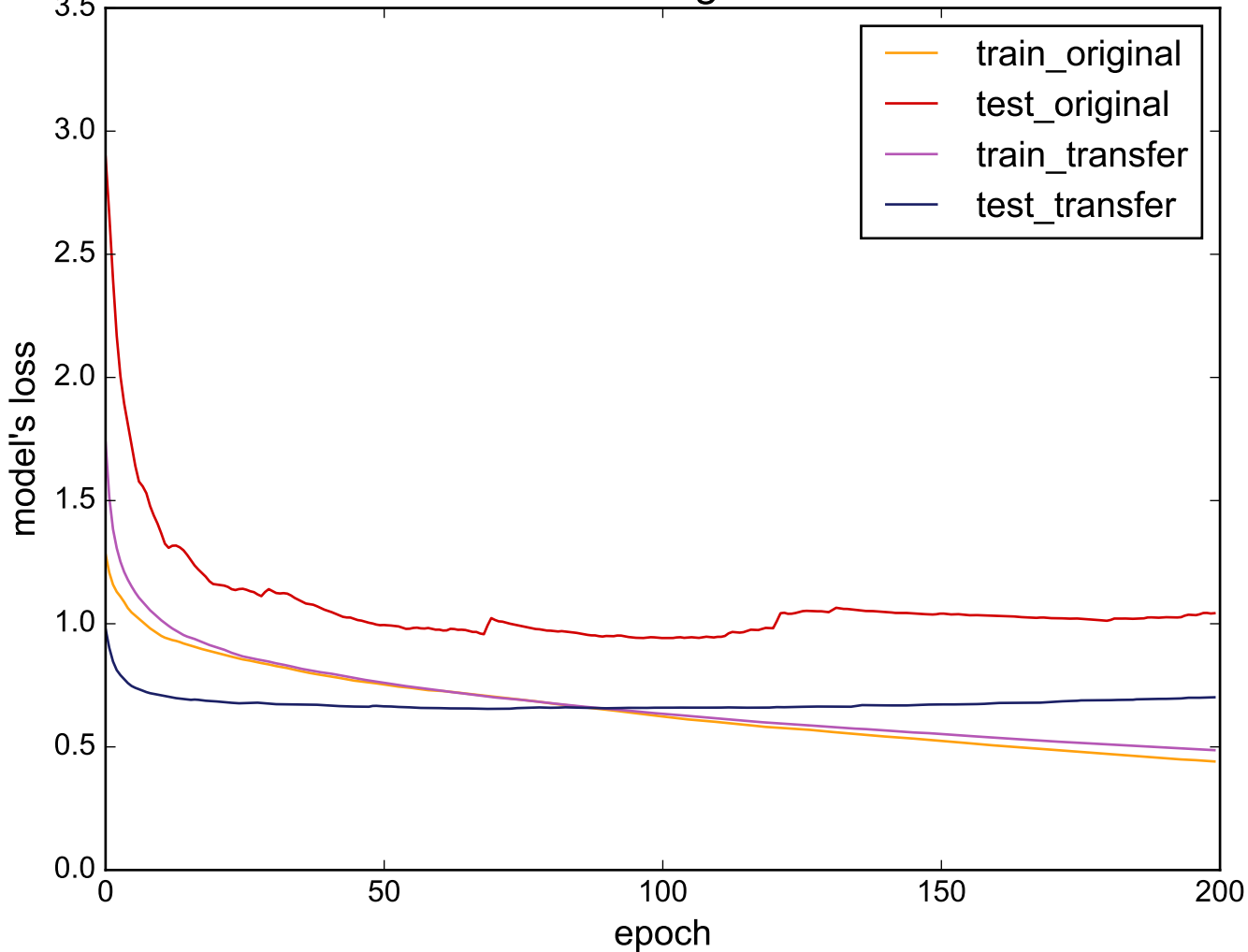
Source: InlineSkate - Target: DistalPhalanxTW
