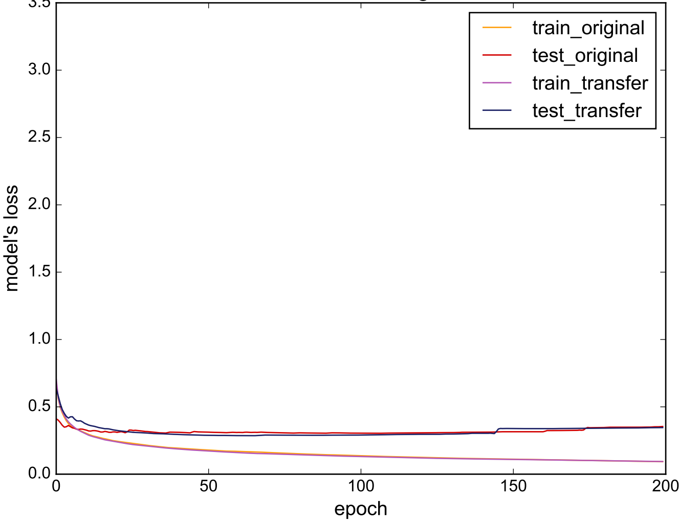
Source: InlineSkate - Target: ECG5000
