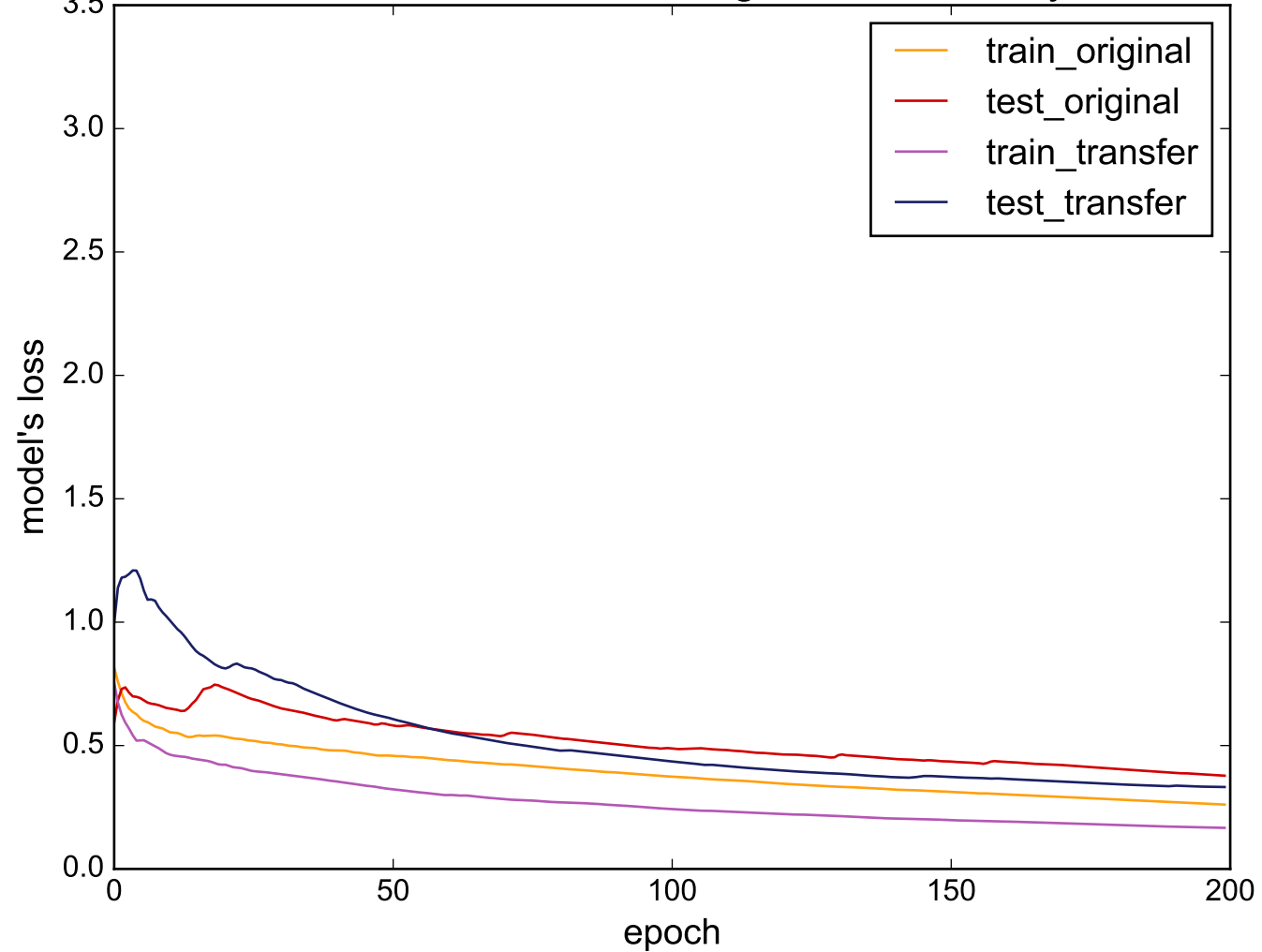
Source: InlineSkate - Target: ECGFiveDays
