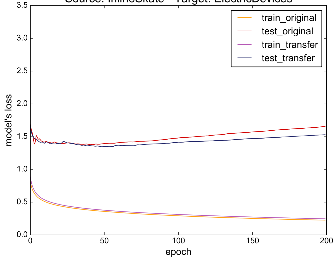
Source: InlineSkate - Target: ElectricDevices
