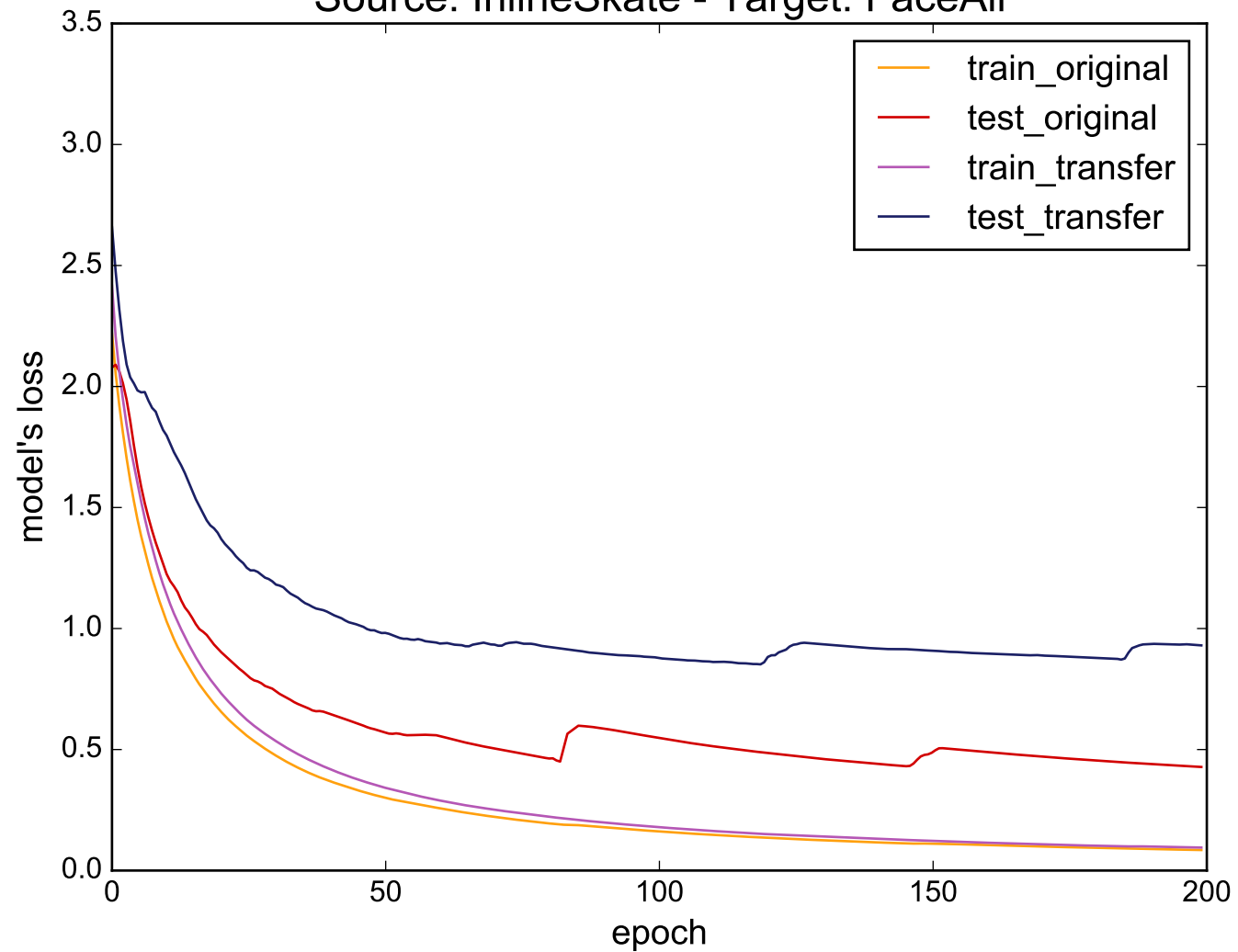
Source: InlineSkate - Target: FaceAll
